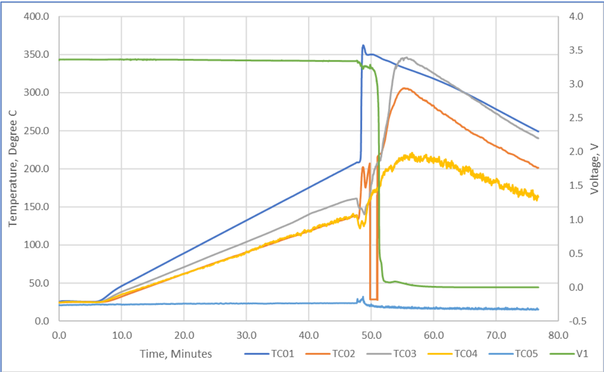
Figure 13: Cell 4 – External Heating 4.3°C per minute
