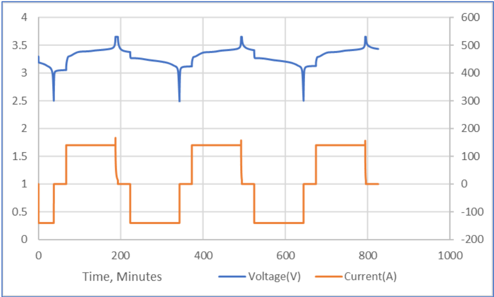
Figure 2: Cell 2 Conditioning (Charge/discharge) Profiles
