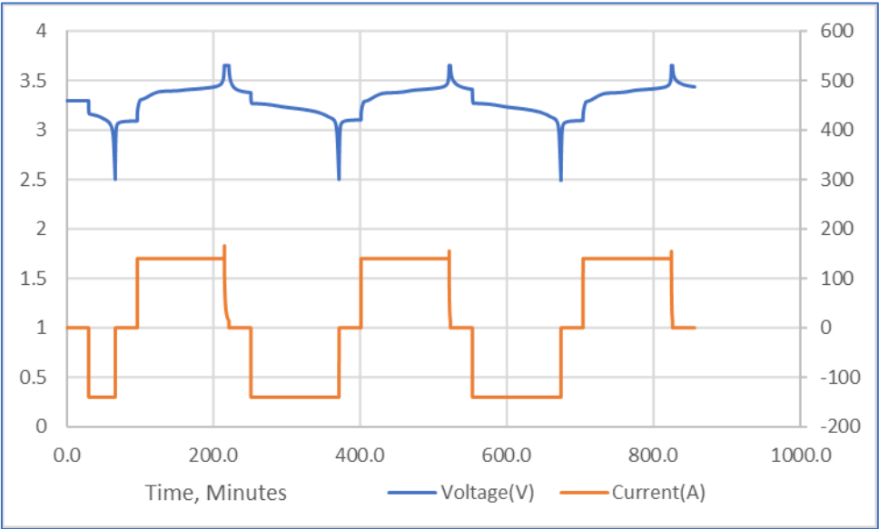
Figure 5: Cell 5 Conditioning (Charge/discharge) Profiles
