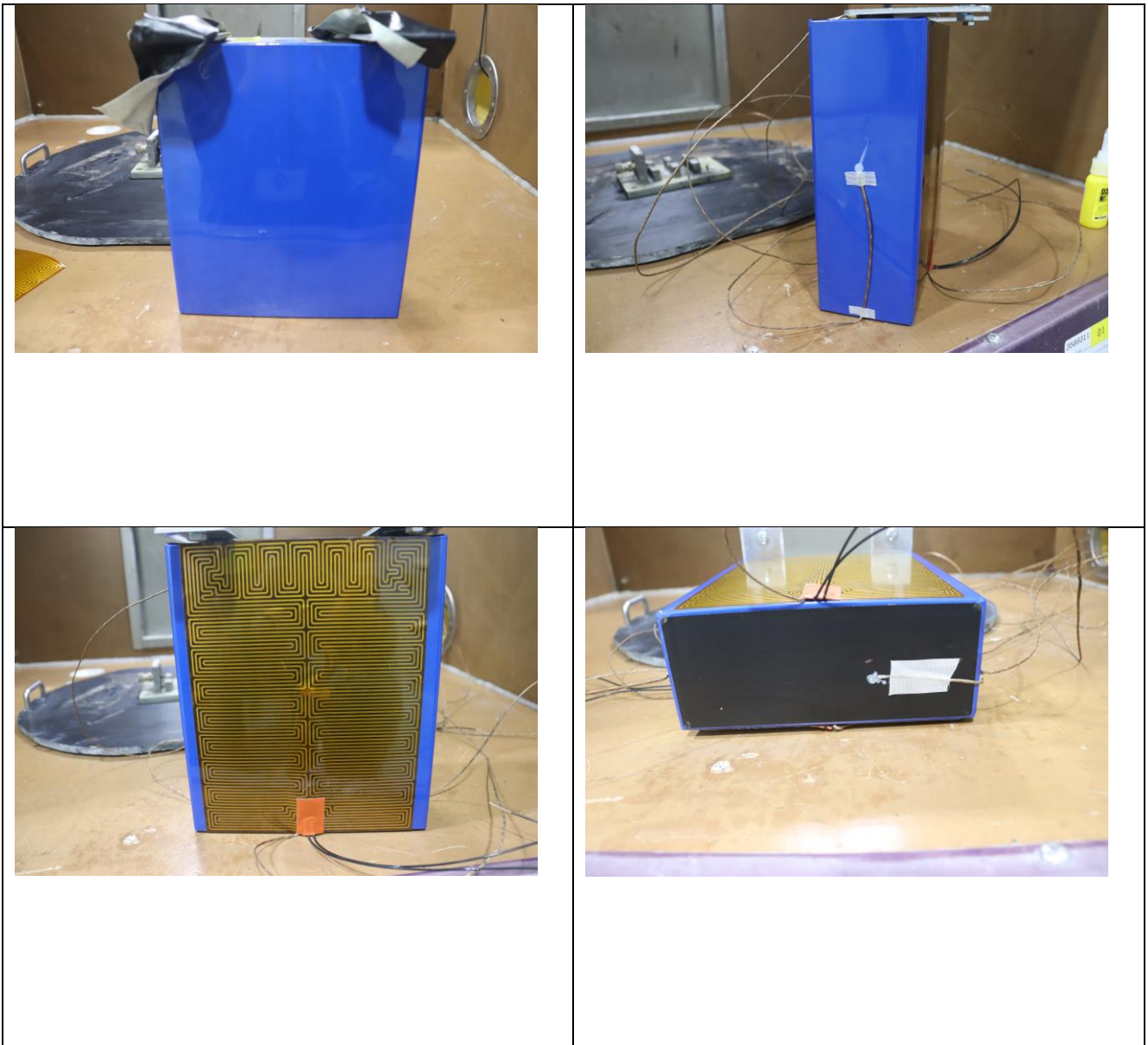
Figure 6: Sample 1 Instrumentation Prior to Test
