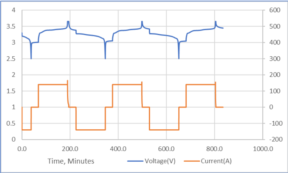
Figure 3: Cell 3 Conditioning (Charge/discharge) Profiles
